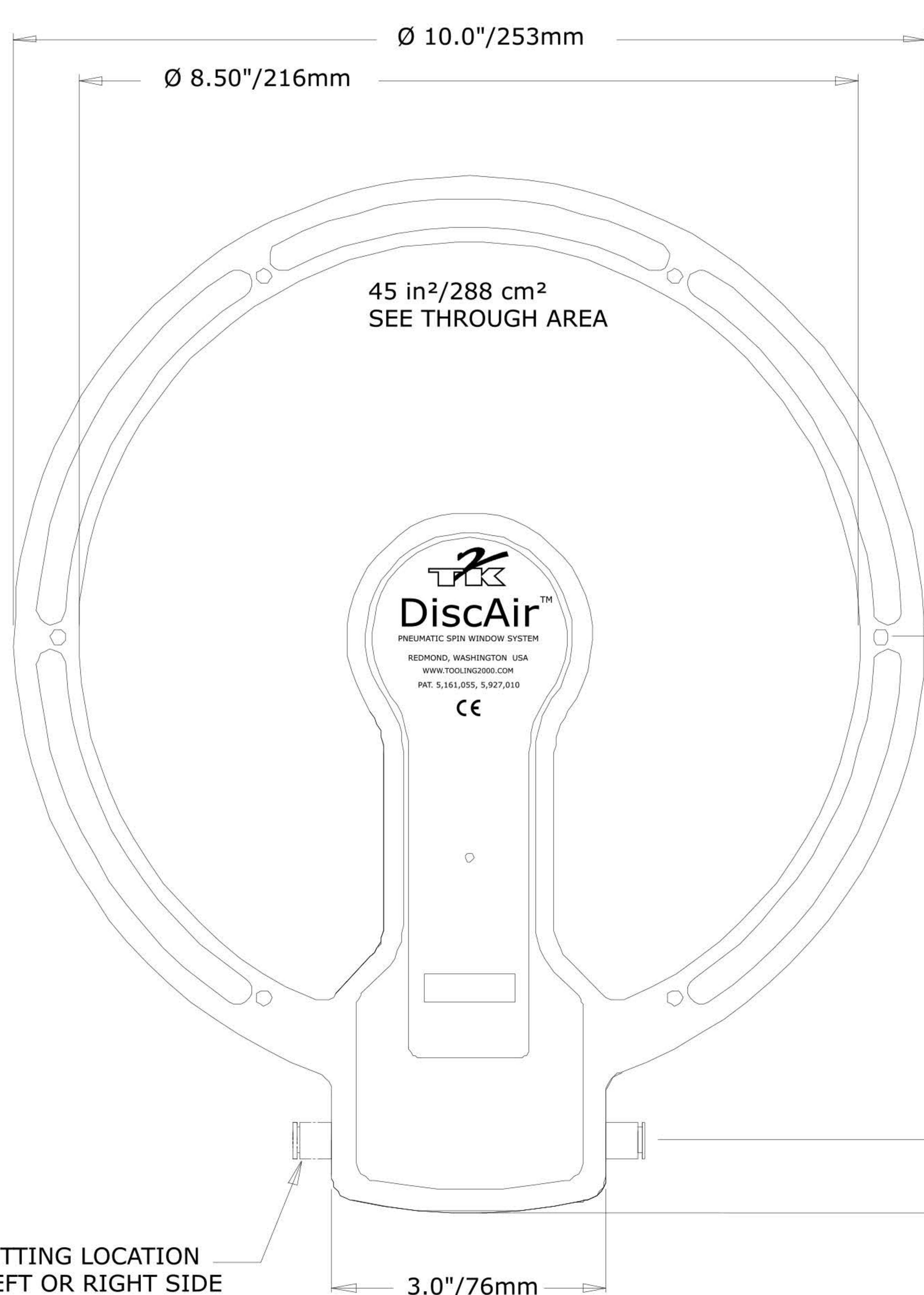
UNIT AS SEEN FROM OPERATOR (DRY) SIDE
